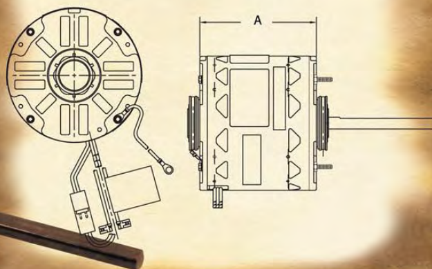
Motor Diagram
